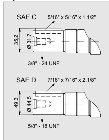
Keyed Shaft
